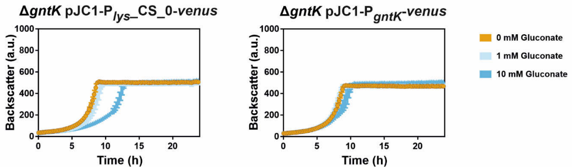
Figure S1: Growth curves corresponding to the analysis of tunability of the native GntR target promoter P_{\text{gntK}} and the synthetic counter-silencer promoter P_{\text{lys\_CS\_0}} shown in Figure 4. Shown are backscatter values of C. glutamicum wild type cells (WT) (A) or C. glutamicum cells lacking the gene encoding the gluconate kinase ( \Delta\text{gntK} ) (B) harbouring the plasmid-based constructs \text{pJC1-P}_{\text{lys\_CS\_0-venus}} or \text{pJC1-P}_{\text{gntK-venus}} during cultivation in the presence of different gluconate concentrations. Graphs show the mean and error bars the standard deviation of biological triplicates over time. Cells were cultivated in a microtiter cultivation system in CGXII medium supplemented with glucose (100 mM in analysis of \text{pJC1-P}_{\text{gntK-venus}} and 111 mM for characterization of \text{pJC1-P}_{\text{lys\_CS\_0-venus}} ) and either no or varying amounts of gluconate as effector. Backscatter values were measured in 15 min intervals. The presented data show that varying amounts of gluconate affect the final backscatter values but did not significantly influence growth rates of wild-type cells. In contrast, \Delta\text{gntK} cells displayed reduced growth rates upon addition of gluconate.
