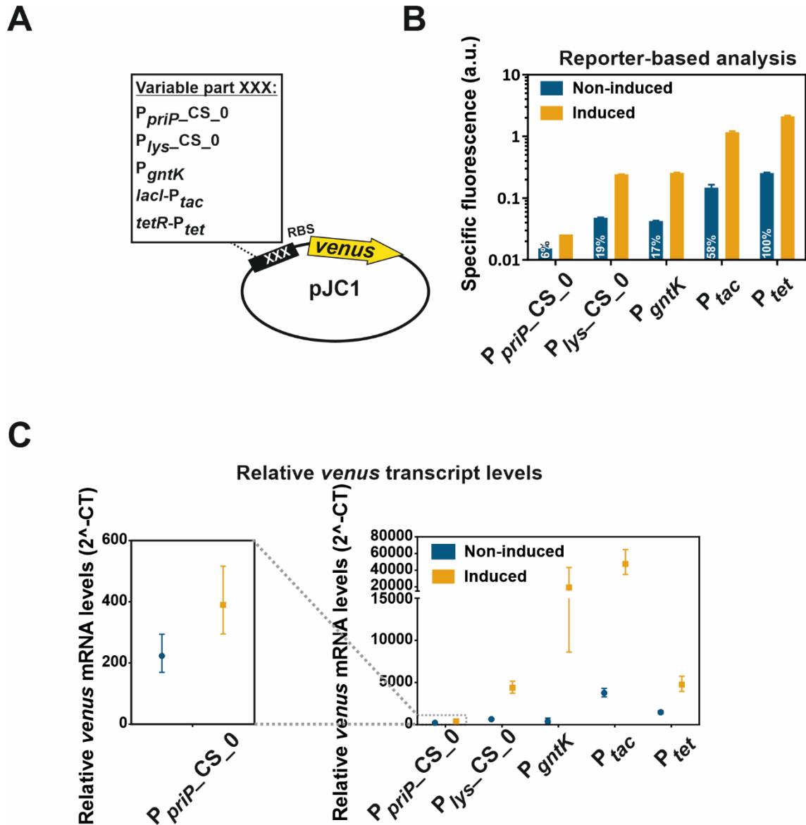
Figure 3: Comparison of counter-silencing constructs with established expression systems.
