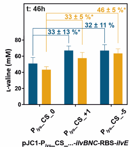
Figure 6: Application of the GntR-dependent toggle for the dynamic switch between growth and L-valine production. A) Schematic representation of relevant parts of the central carbon metabolism and the L-valine biosynthesis pathway of C. glutamicum . The GntR-dependent
